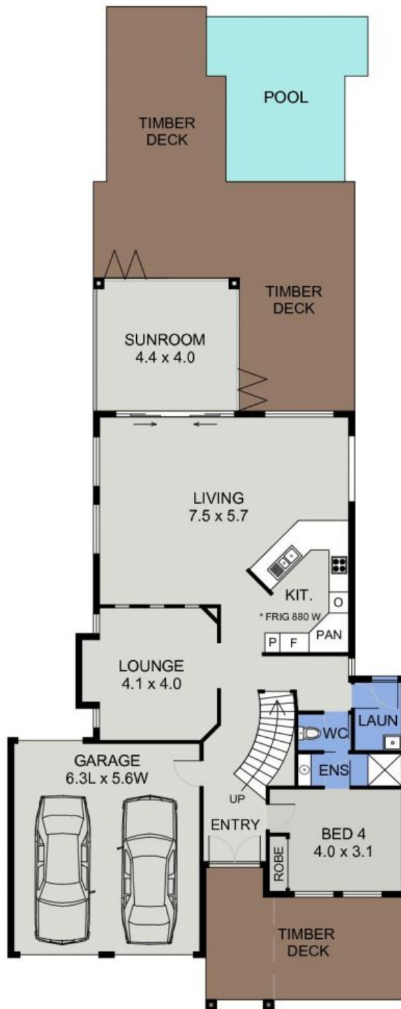
LOWER FLOOR PLAN ( 169 sq m Approx )
