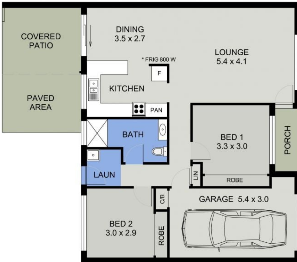
FLOOR PLAN ( 99 sq m Approx )
