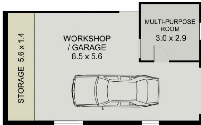
GARAGE PLAN
