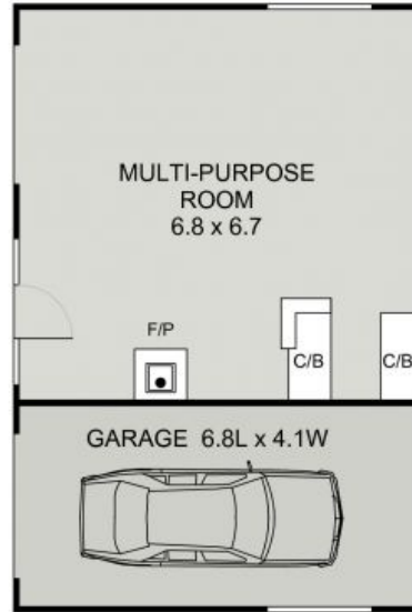
GARAGE FLOOR PLAN
