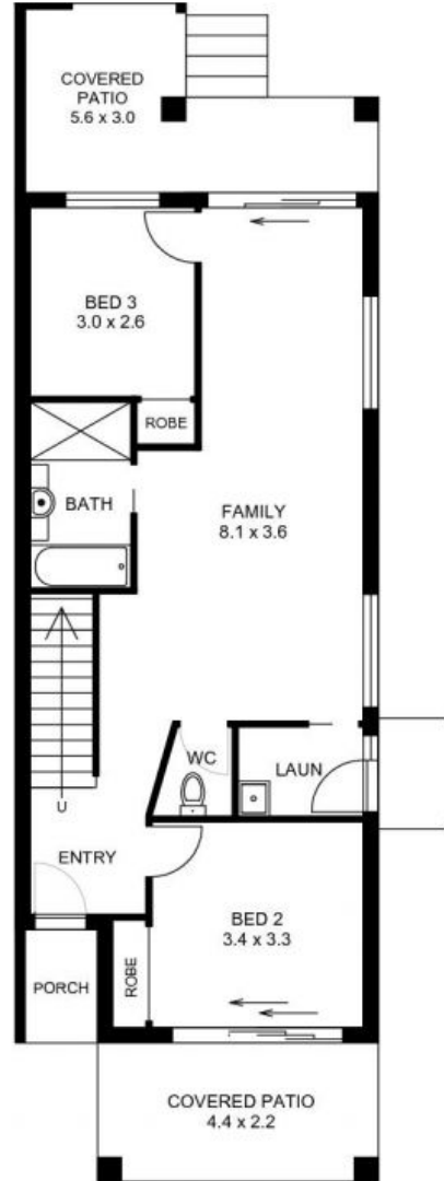
LOWER FLOOR PLAN ( 73 sq m Approx )
