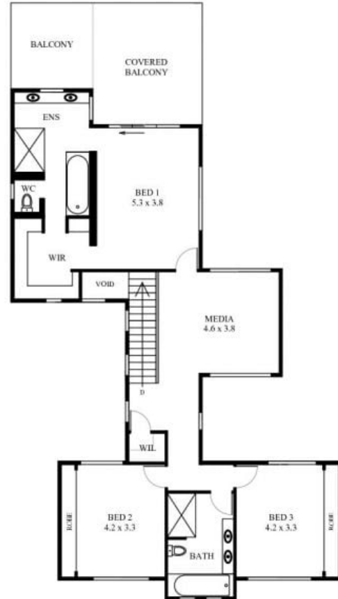
UPPER FLOOR PLAN (130 sq m Approx.)
