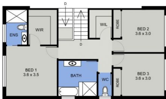
UPPER FLOOR PLAN ( 74 sq m Approx )
