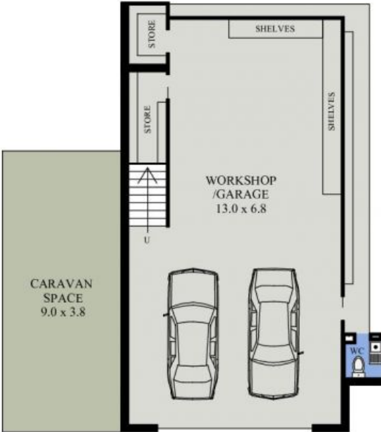
LOWER FLOOR PLAN (95 sq m Approx)
