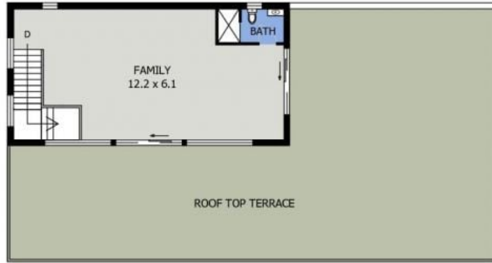
UPPER FLOOR PLAN ( 82 sq m Approx )
