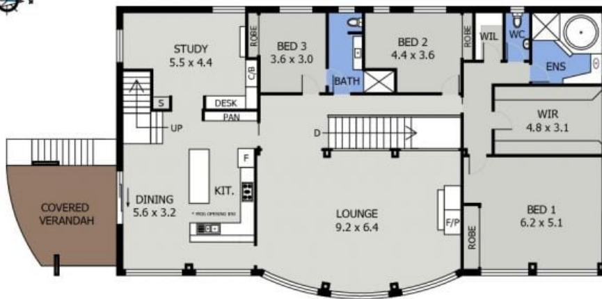
MIDDLE FLOOR PLAN ( 274 sq m Approx )
