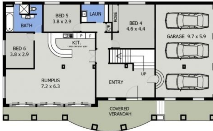
LOWER FLOOR PLAN ( 233 sq m Approx )
