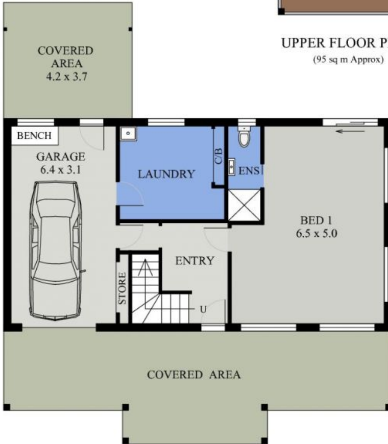
LOWER FLOOR PLAN (87 sq m Approx)
