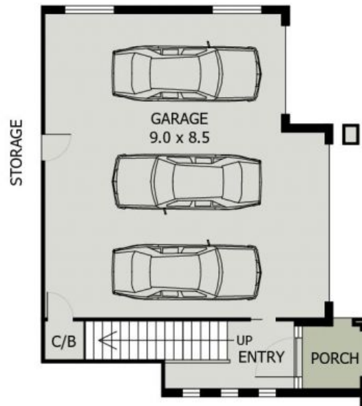
LOWER FLOOR PLAN ( 95 sq m )
