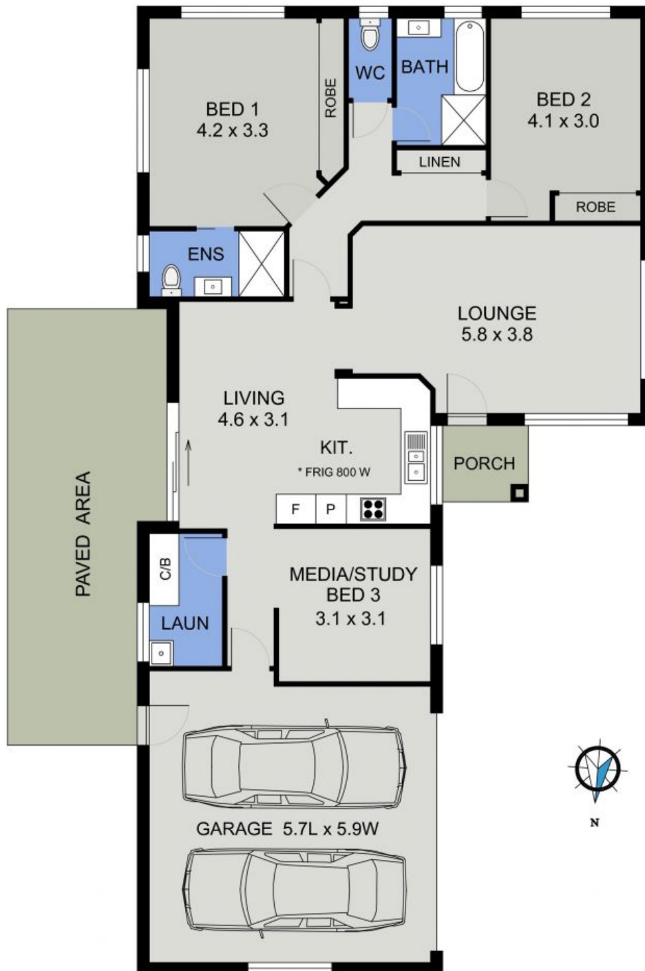
FLOOR PLAN (154 sq m Approx)
