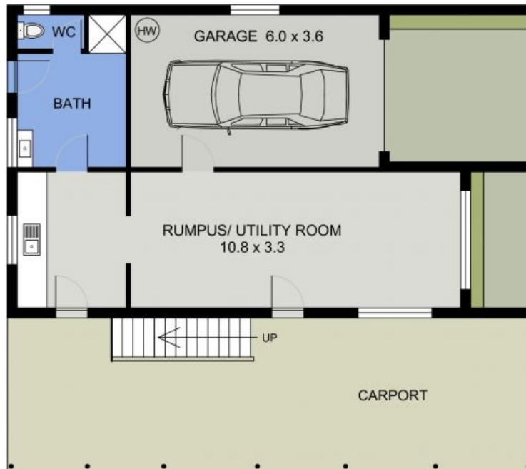
LOWER FLOOR PLAN (79 sq m Approx)
