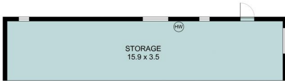
LOWER FLOOR PLAN (61 sq m Approx)
