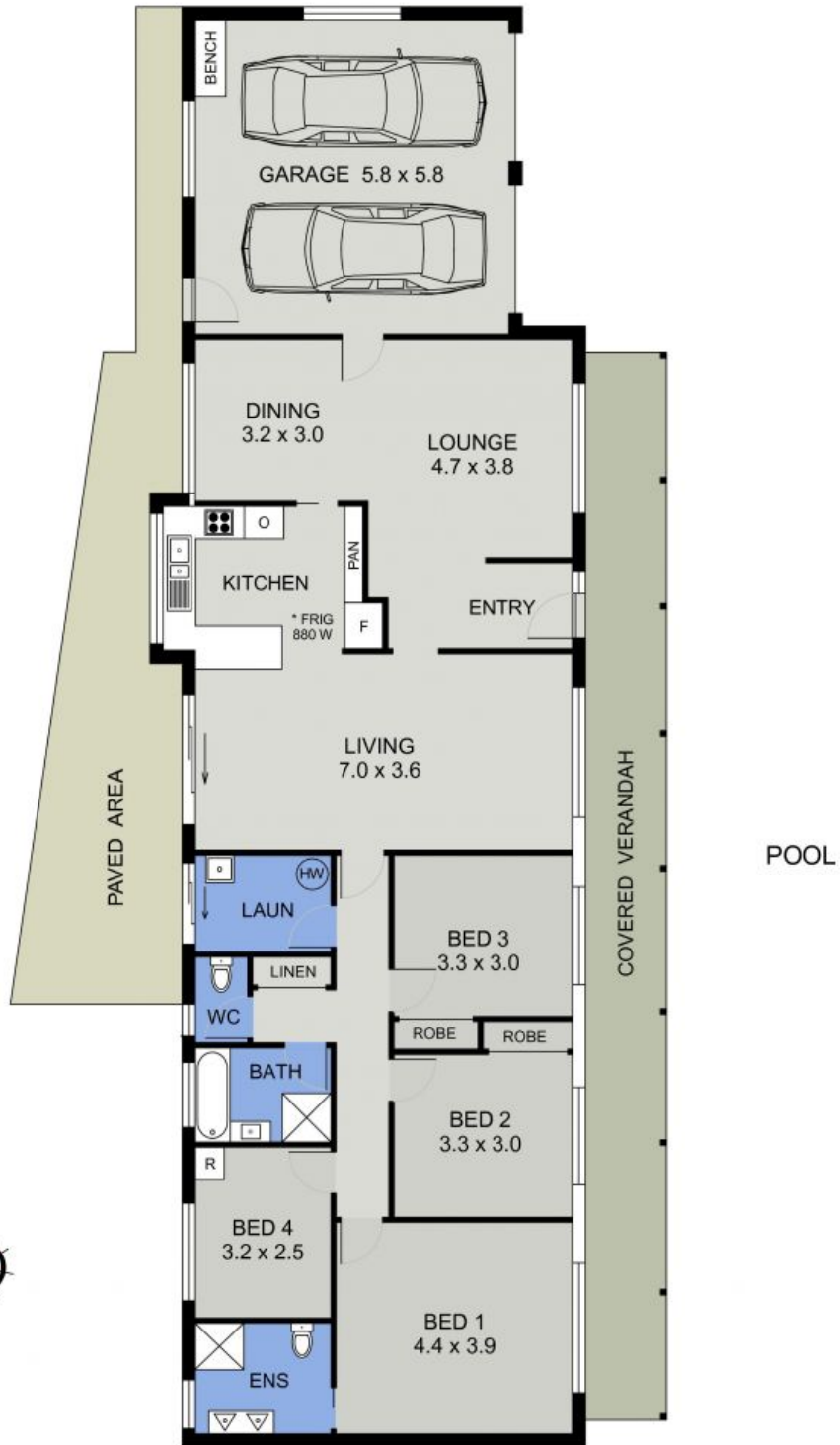
FLOOR PLAN (194 sq m Approx)
