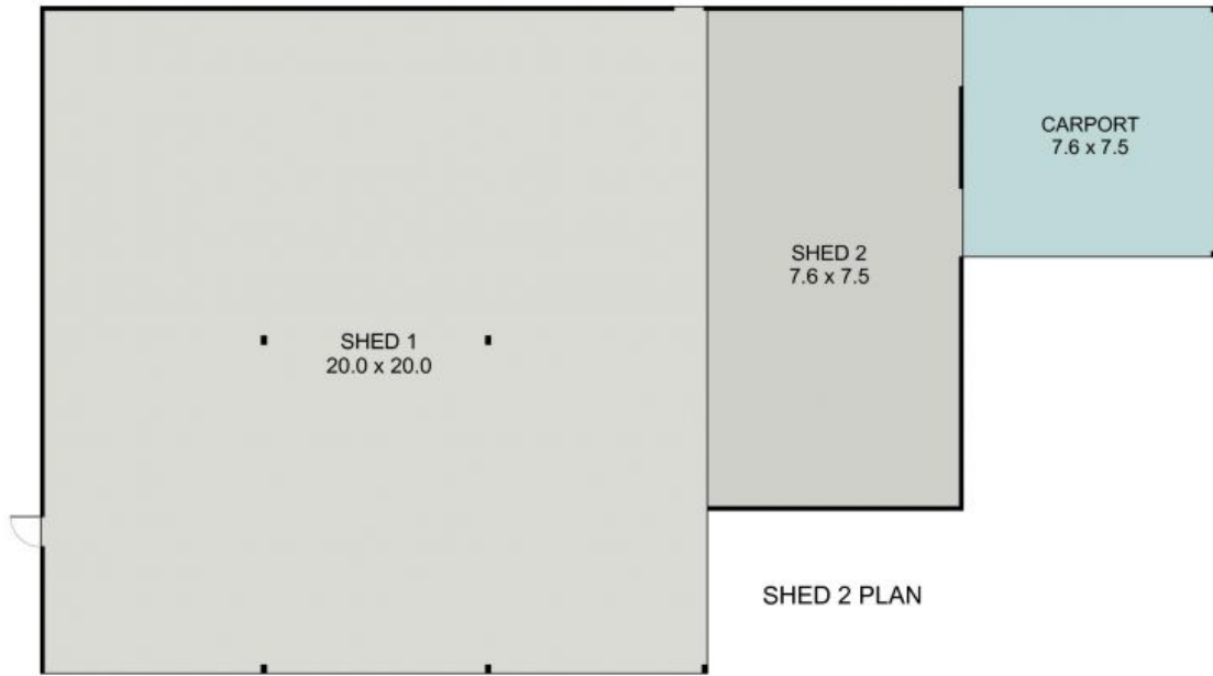
SHED 1 PLAN
