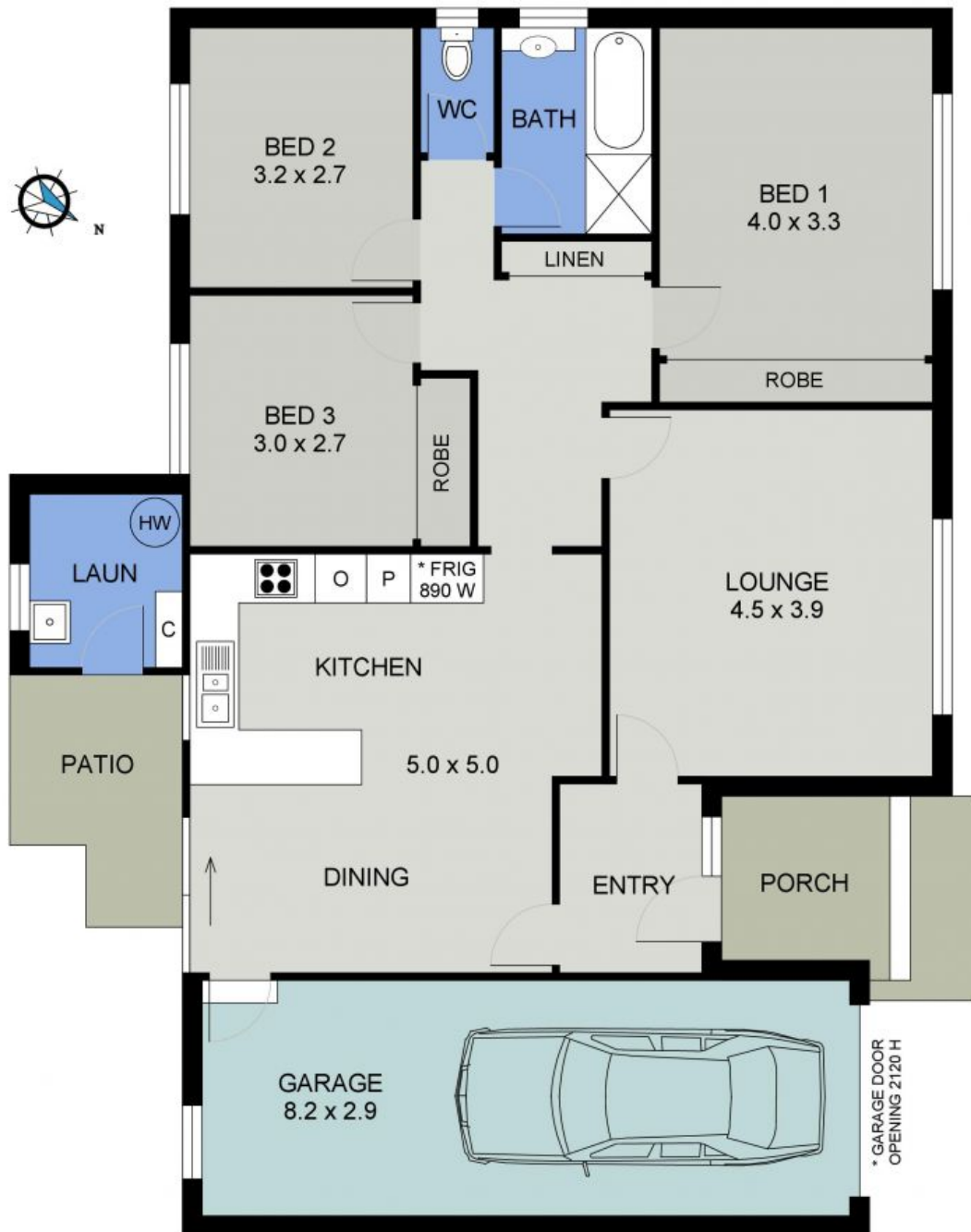
FLOOR PLAN ( 138 sq m Approx )
