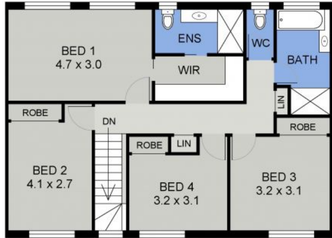
UPPER FLOOR PLAN ( 84 sq m Approx )
