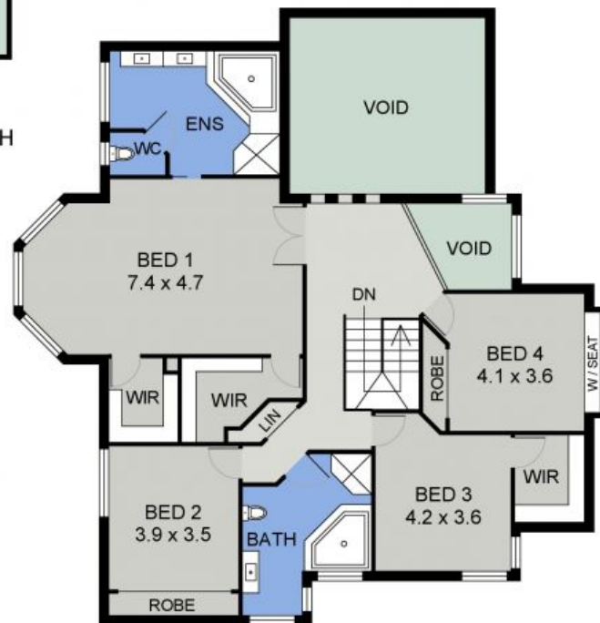
UPPER FLOOR PLAN (153 sq m Approx) Scale - 1:140
