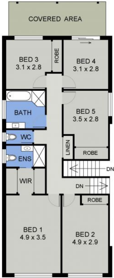
UPPER FLOOR PLAN (103 sq m Approx)
