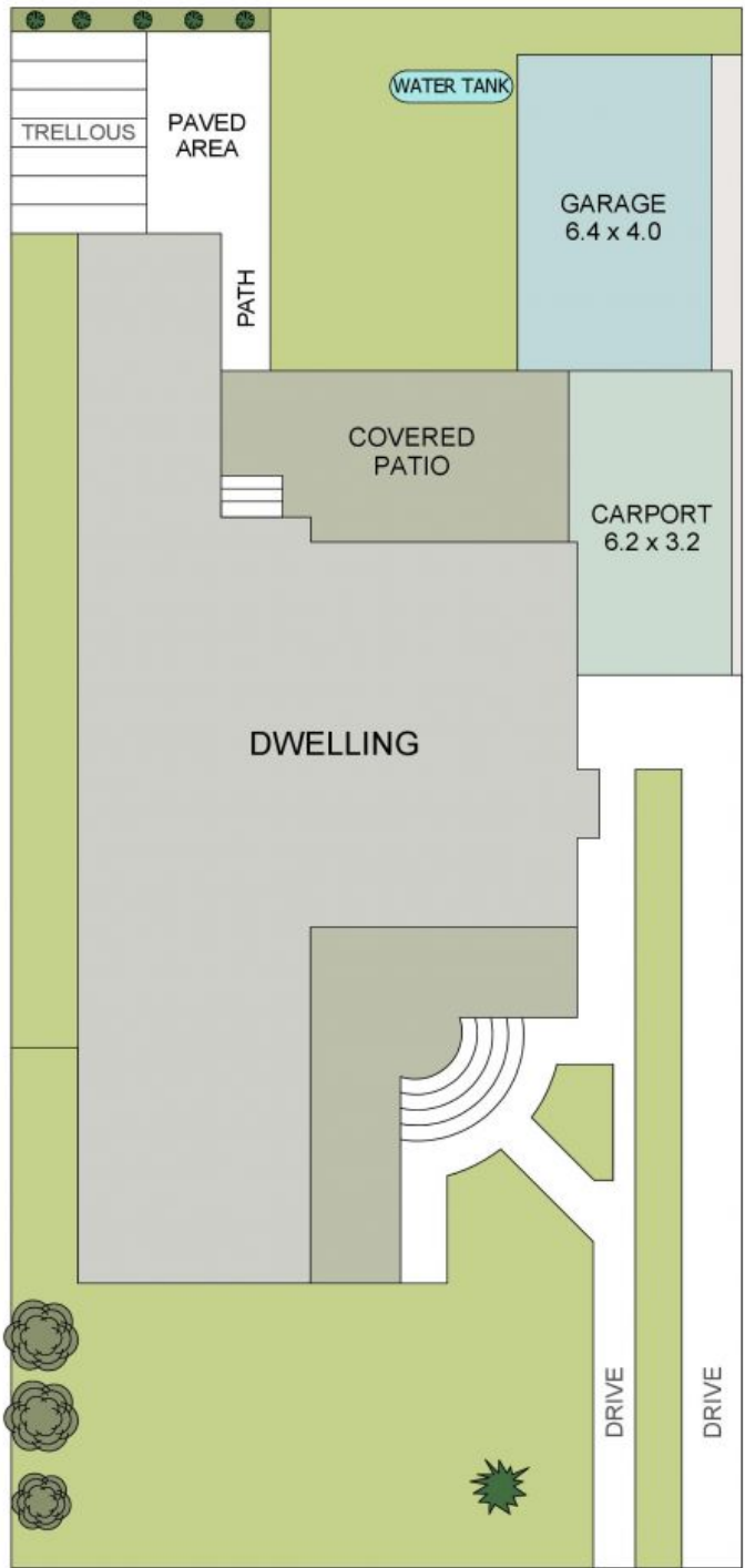
SITE PLAN (486.9 sq m) Approx) Scale - 1:130
