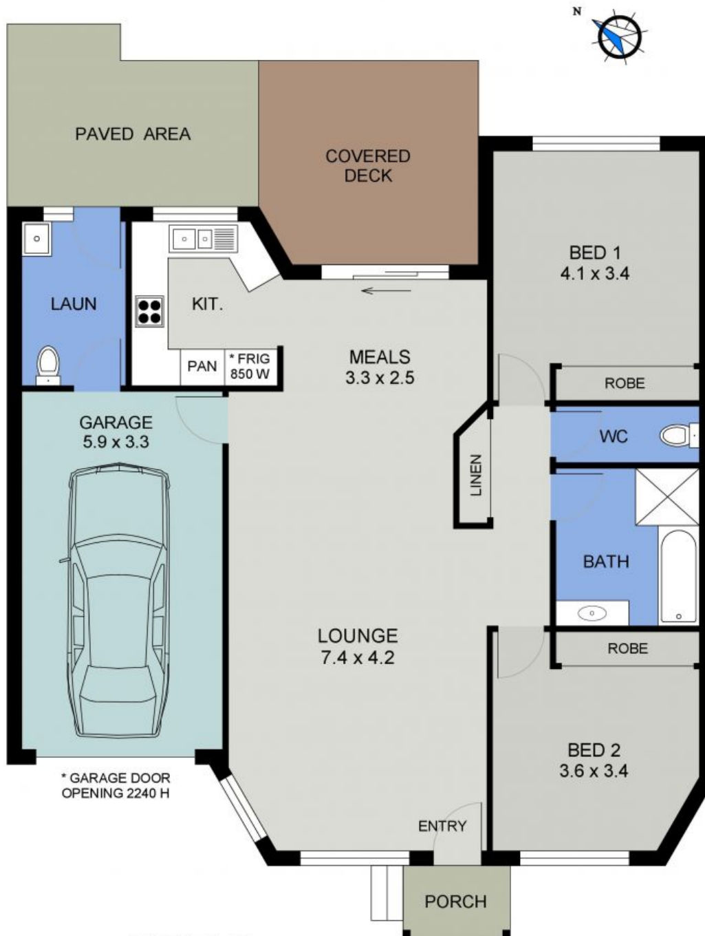
FLOOR PLAN ( 116 sq m Approx ) ( Scale: 1:65 )
