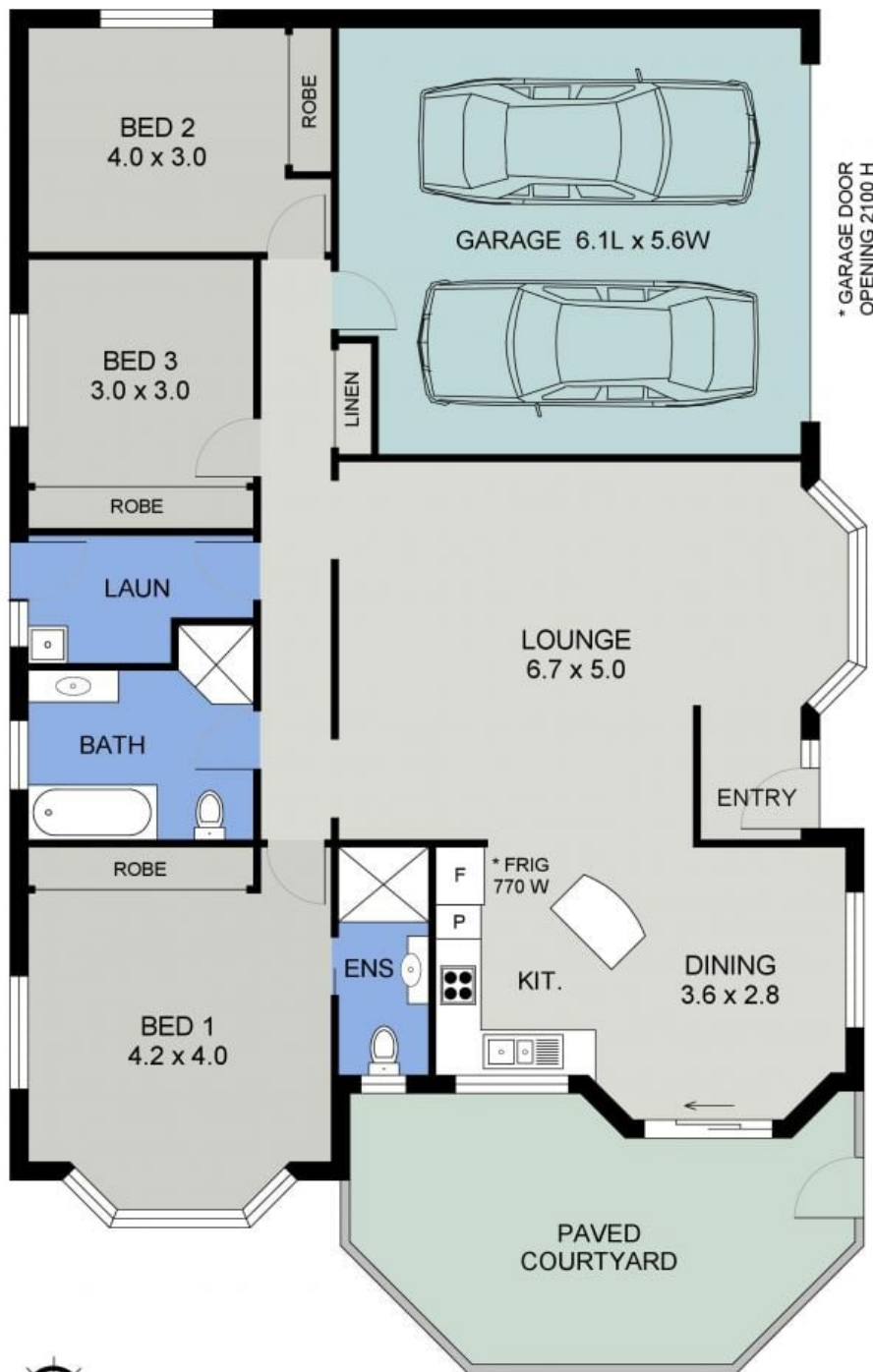
FLOOR PLAN (167 sq m Approx) Scale - 1:75
