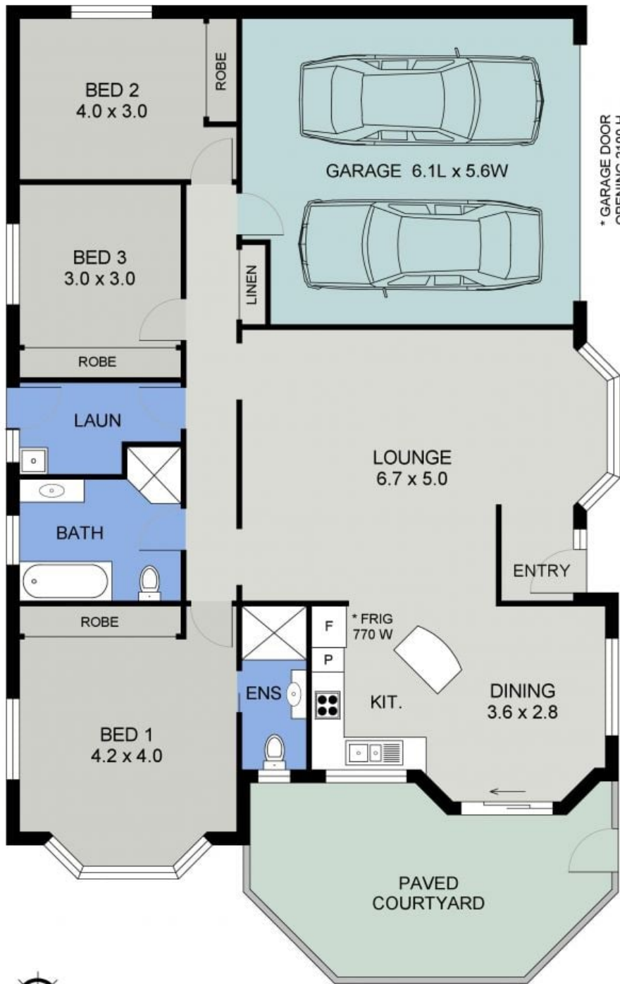
FLOOR PLAN (167 sq m Approx) Scale - 1:75
