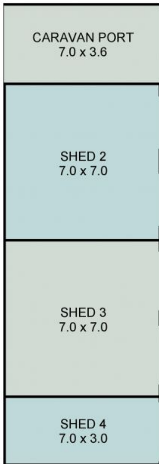
SHEDS 2,3,4 PLANS (125 sq m Approx) Scale - 1:130
