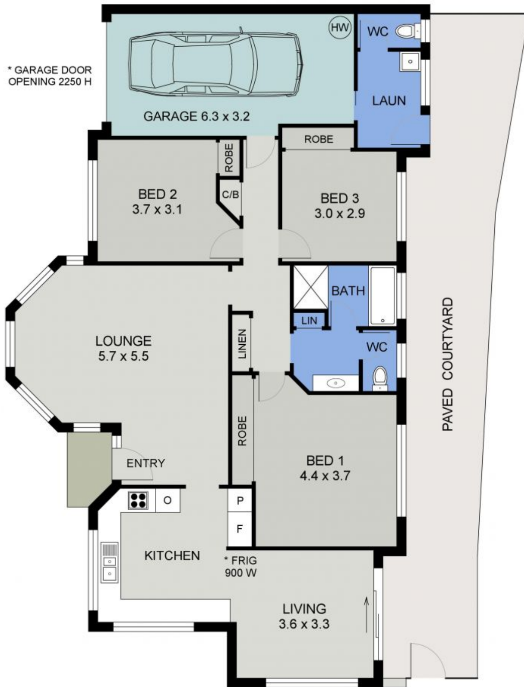
FLOOR PLAN (145 sq m Approx) Scale - 1:75
