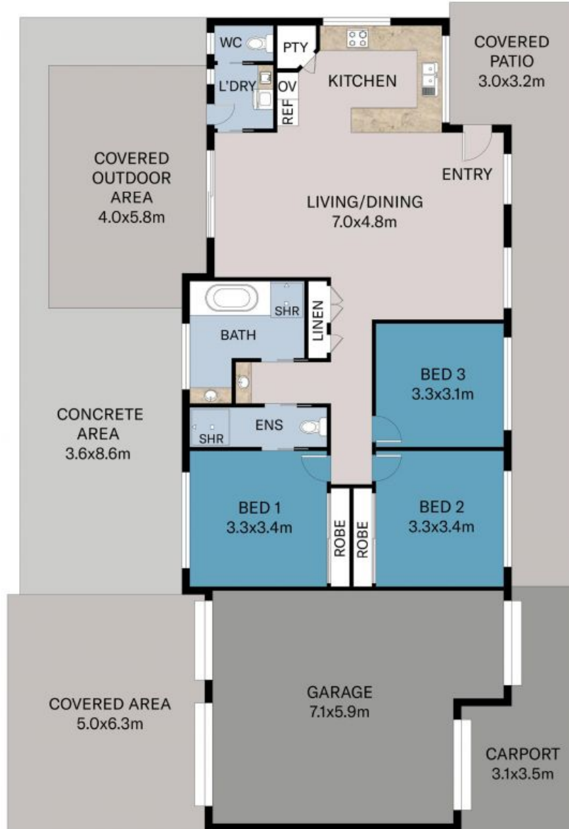
FLOOR PLAN
