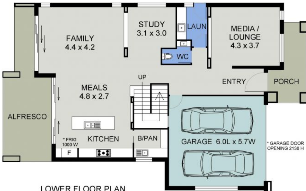
LOWER FLOOR PLAN (187.7 sq m) Scale - 1:110
