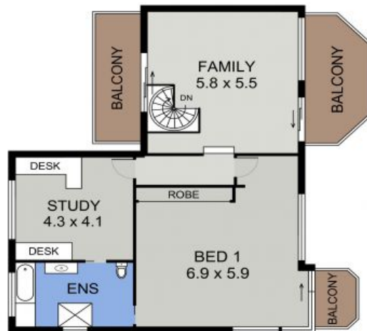
UPPER FLOOR PLAN (116 sq m Approx) Scale - 1:150
