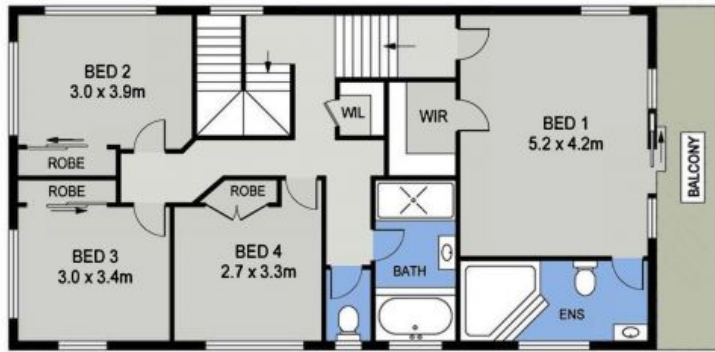
UPPER PLAN (103 sq m Approx)
