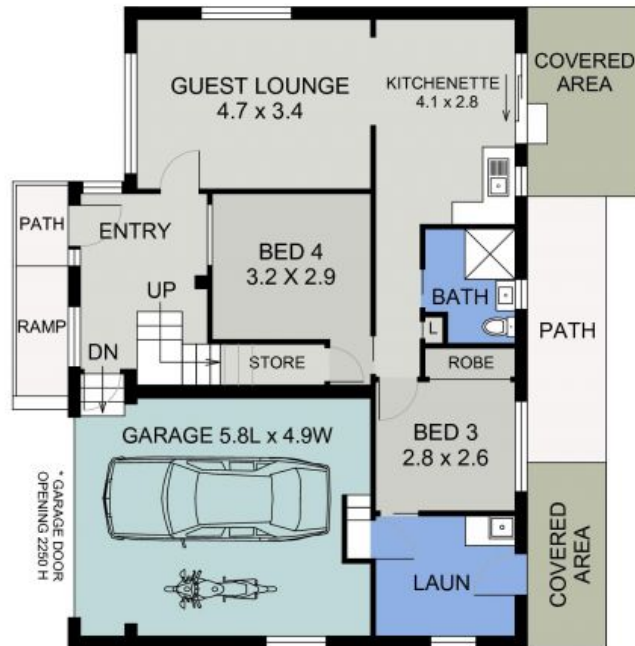
MIDDLE FLOOR PLAN (113 sq m Approx)
