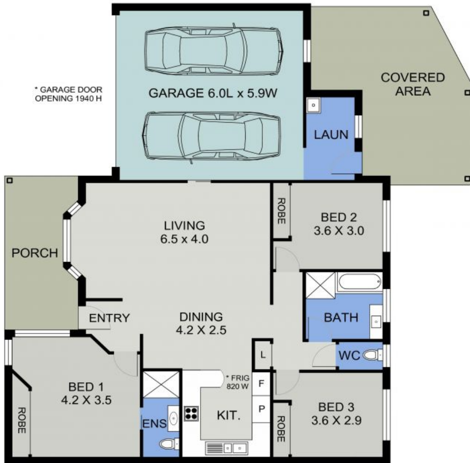
FLOOR PLAN (158 sq m Approx) Scale - 1:85
