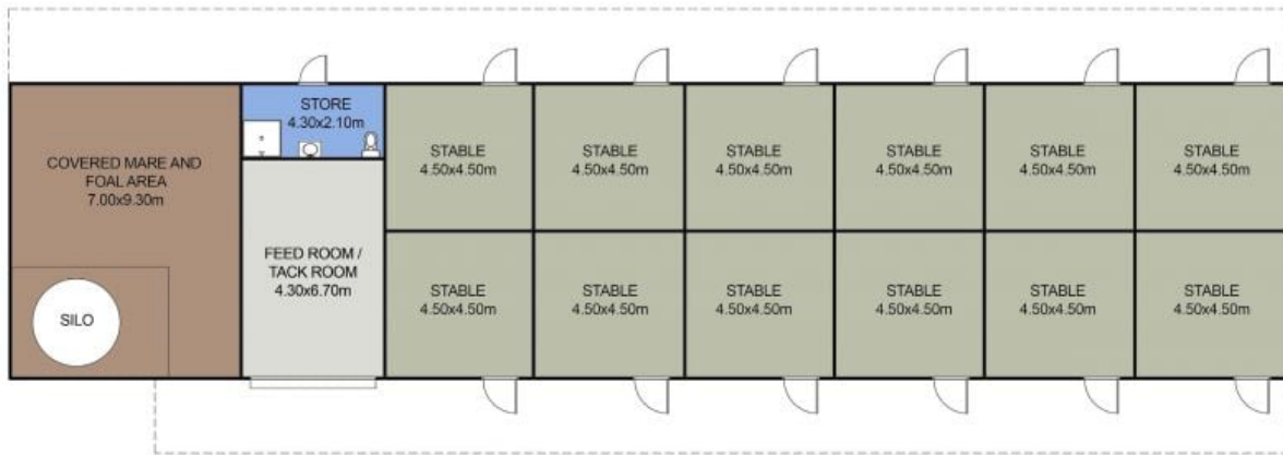
FLOOR PLAN
